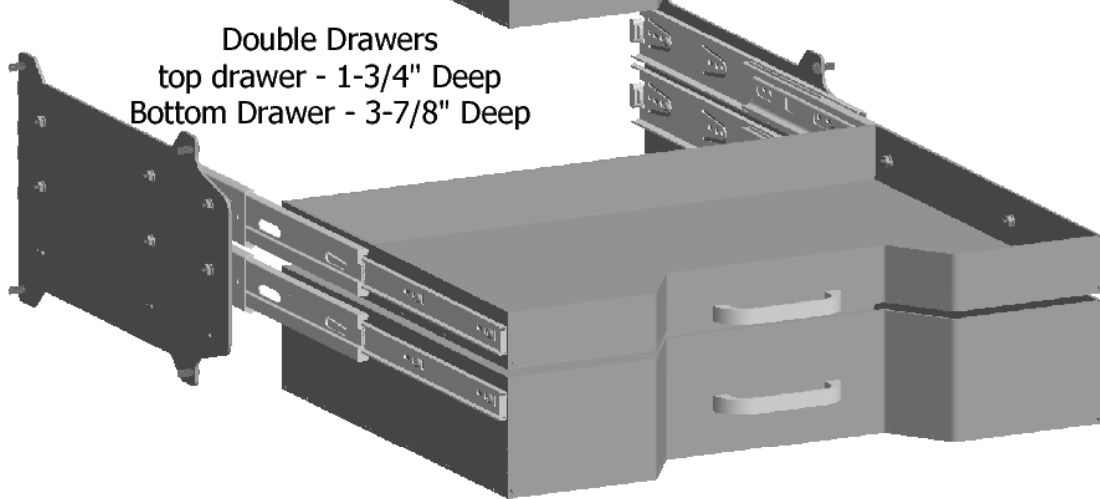
Triple Drawers All drawers - 1-3/4" Deep
