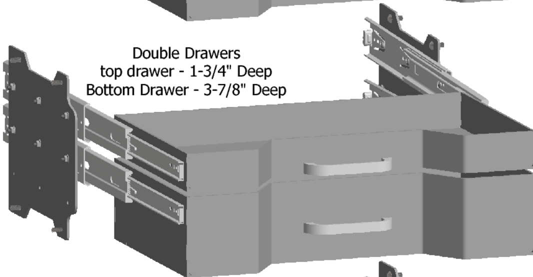
Triple Drawers All drawers - 1-3/4" Deep
